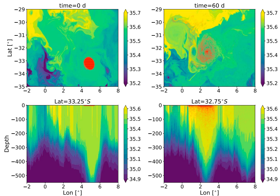
Figure 16. An expanding rotatorily coherent Lagrangian vortex (RCLV): Snapshots of the initial (left) and final (right) positions of 3-D particles with the same initial positions as RCLV 1 (left column of Figure 15) advected off-line by hourly velocities superimposed on salinity concentration in the region from online llc4320 simulation output. The colors in the top panels show the salinity at the surface. The bottom panels show a cross section (taken along a latitude line, across the eddy) of the salinity field, and the particles are shown in red. The salinity column marked by the eddy extends to a shallower depth at 60 days, which indicates possible upwelling inside the eddy core. Based on the salinity stratification and the fact that the RCLV expands with time (expansion => upwelling inside), we can reasonably infer that there is possible upwelling inside the eddy core.
